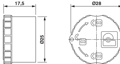
Dimensional drawing
